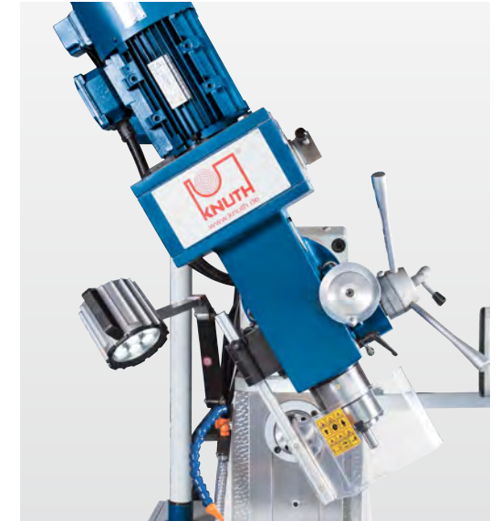
Swiveling head quill
